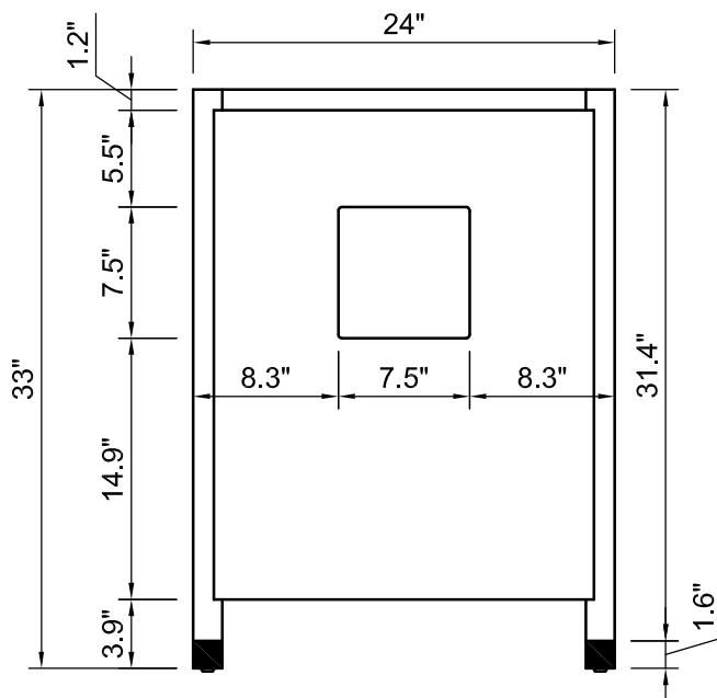
BACK VIEW
